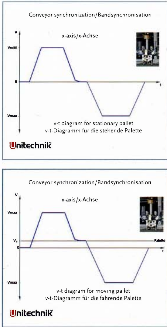
Fig. 2 Conveyor synchronization for stationary and for continuously moving pallet.
